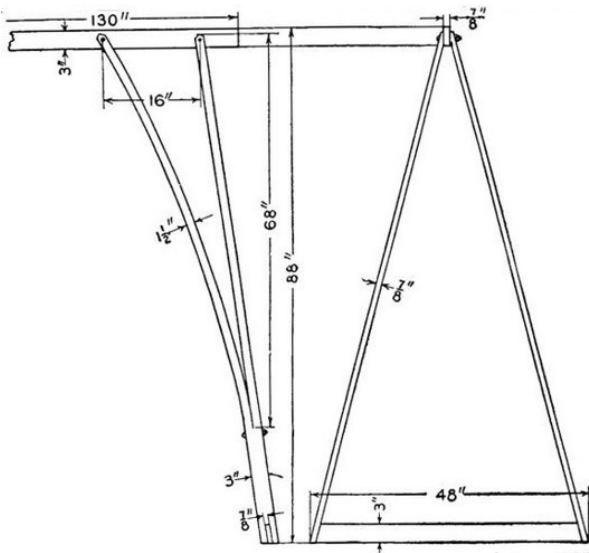
Showing Construction of Stand
