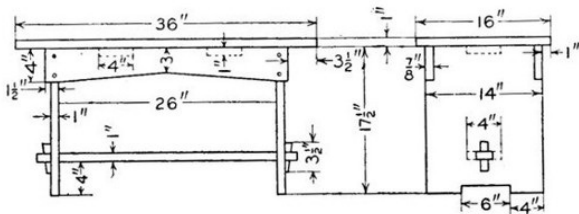
Piano Bench Details
