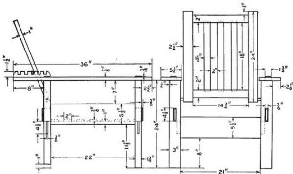
Details of a Morris Chair
