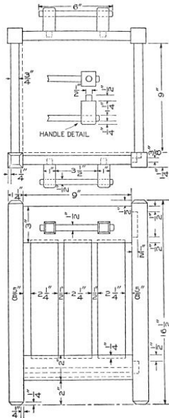
Detail of Waste-Paper Basket
