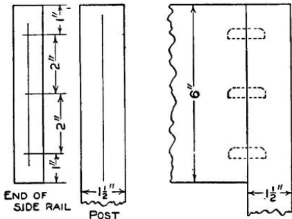
Details of Shoe Rest
