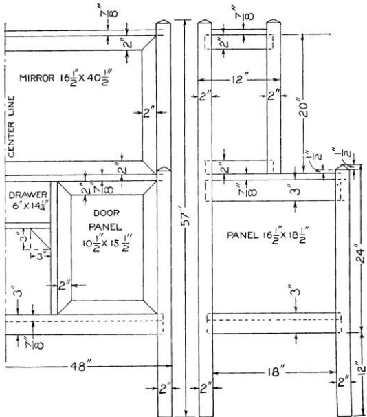
Detail of the Mission Sideboard
