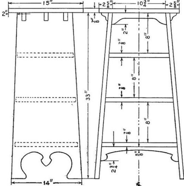
Details of the Magazine Stand
