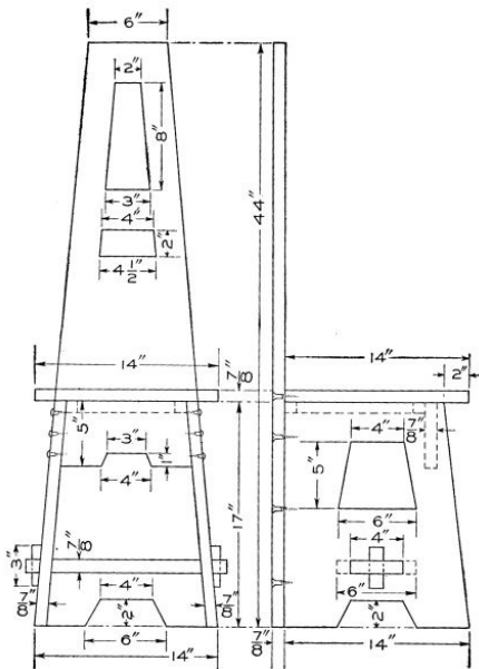
Detail of the Hall Chair
