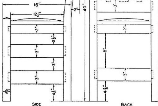
Details of Chair Construction
