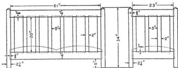
Details of a Mission Settee
