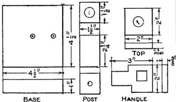
Details of Candlestick
