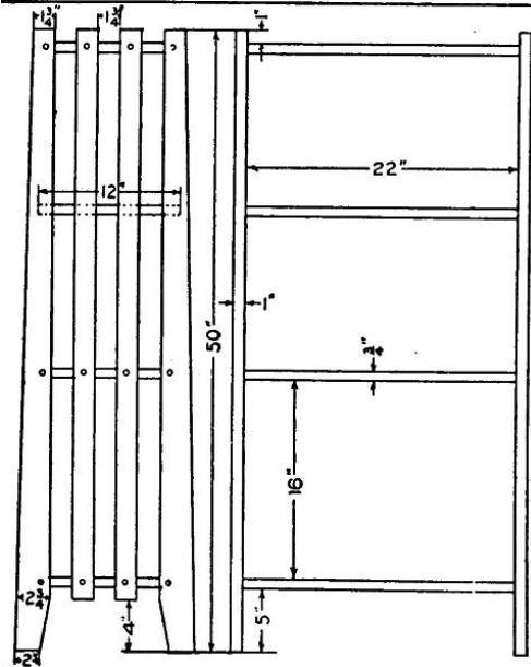
Details of Stand
