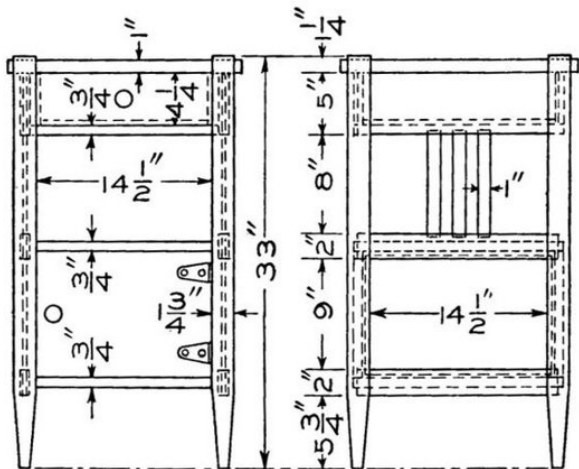
Detail of the Medicine Stand
