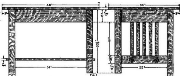
Showing Dimensions of Table
