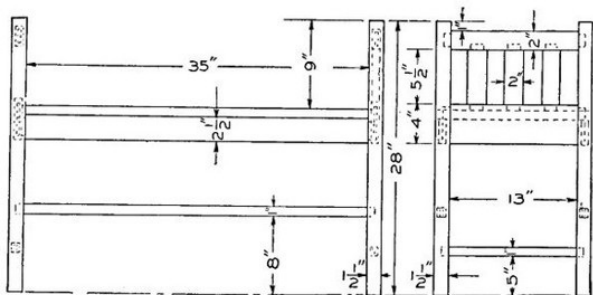
Detail of the Hall or Window Seat
