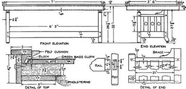
Details Showing Dimensions of Parts
