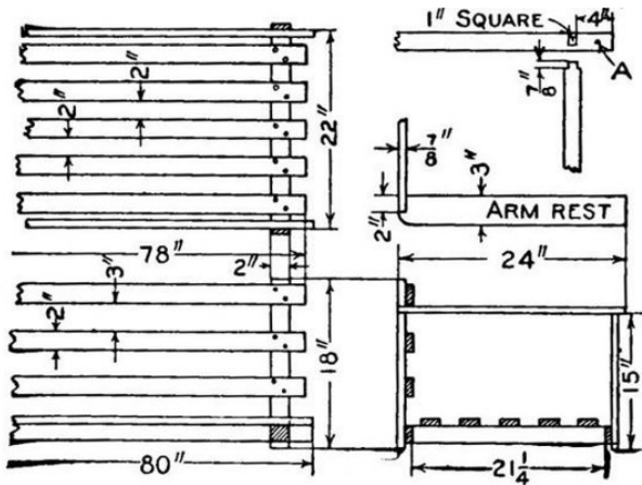
Details of Seat
