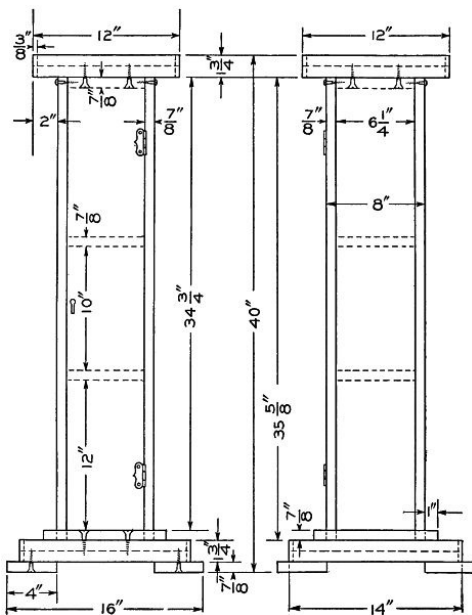
Detail of Cellarette Pedestal
