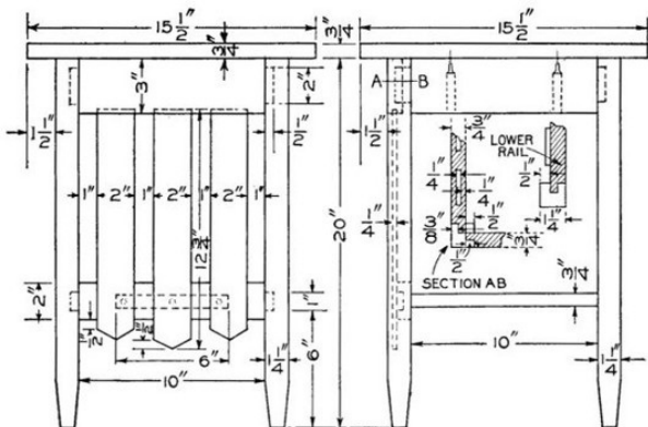
Detail of the Plant Stand
