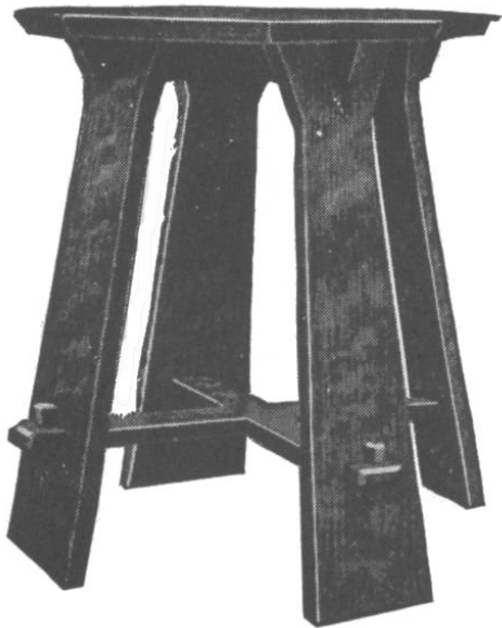
Tabouret as Completed
