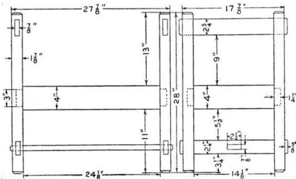
Details of Parts of Chair
